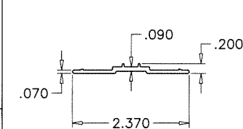
E34 VERTICAL SUPPORT
