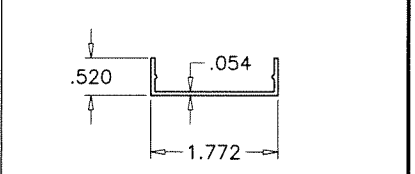
E26 CORNER COVER
