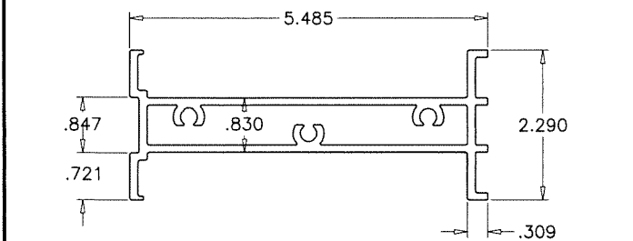
E07 SHEAR BLOCK
