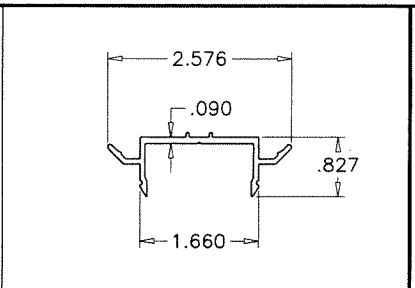
E21 VERTICAL CORNER SUPPORT
