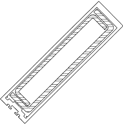
CORNER MULLION
