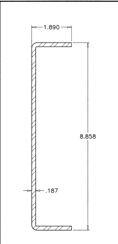
M30 REINF. CHANNEL (JAMB)
