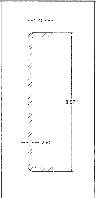
M31 REINF. CHANNEL (MULLION)
