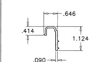
E34 VERTICAL SUPPORT
