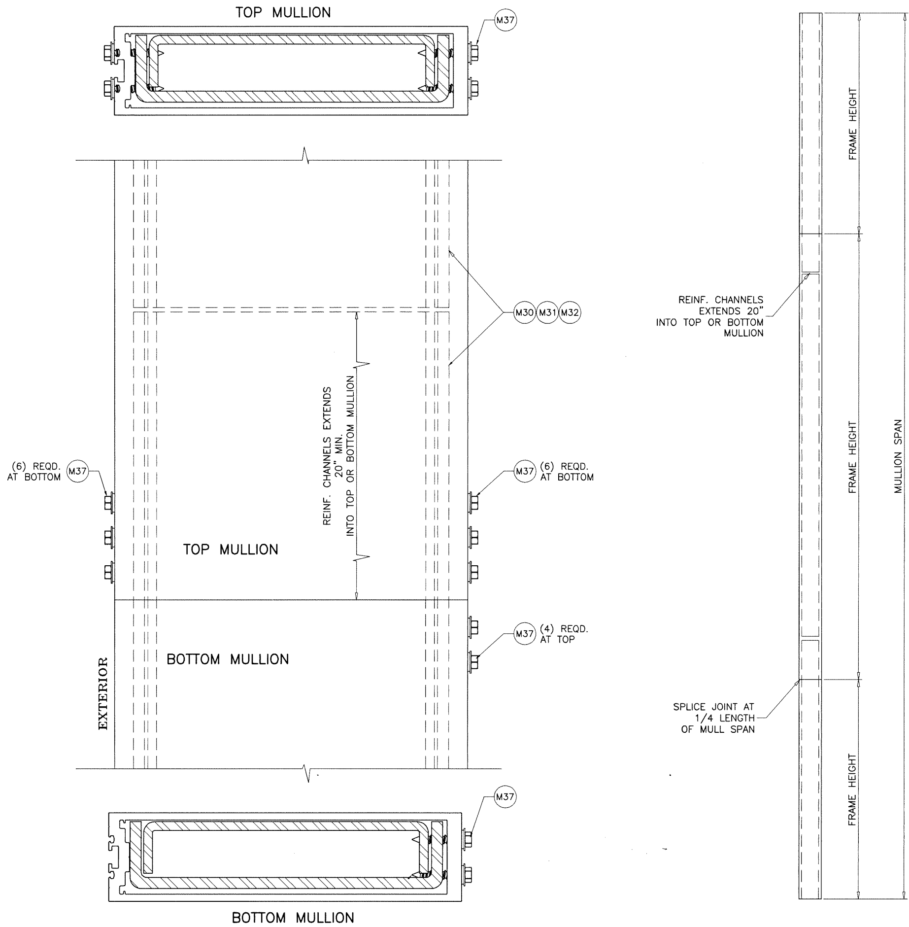
JAMB & MULLION JOINT
